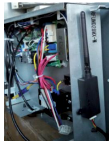
Radio adapter for the indoor unit to be connected to the respective electronic board.
